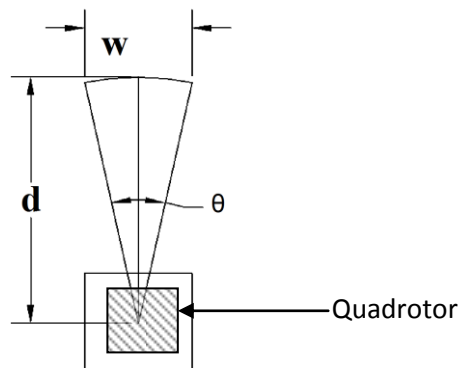
Figure 2: Obstacle Scanning Range
